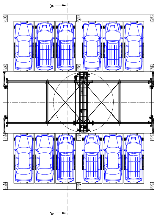
TYPICAL FLOOR
