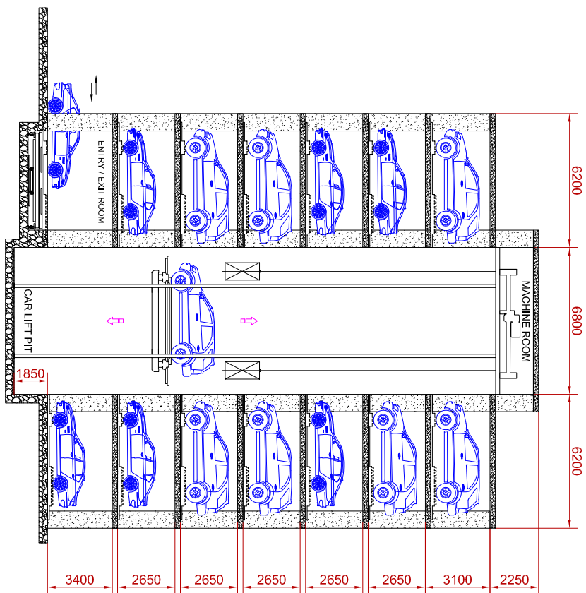
TYPICAL FLOOR
